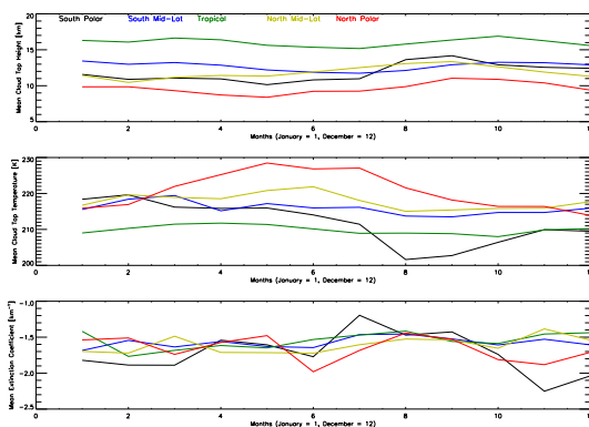
Figure 12. Time series for CTH (top), CTT (middle) and \log(k_{ext}) (bottom) for the full year of 2003 from MIPAS.
