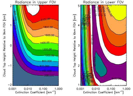
Figure 5. Radiance measured in the upper and lower fields-of-view, where cloud is first encountered. Here the cloud top is given in kilometers above a 9 km tangent height.
