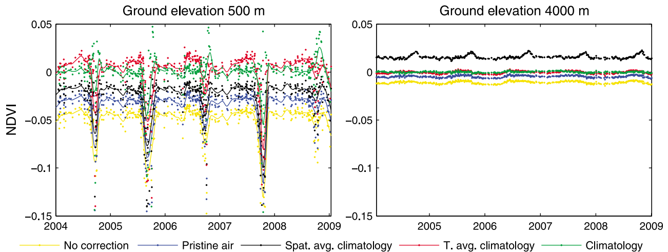
Figure 8. Atmospheric bias of green vegetation NDVI (0.63) at low ( 500 \pm 250 m) and high ( 4000 \pm 250 m) ground elevation. (left) The vertical axis was cropped for better data visualization (NDVI bias range, -0.15 to -0.4 ; 21 points omitted). See the caption of Figure 6 for further information.
